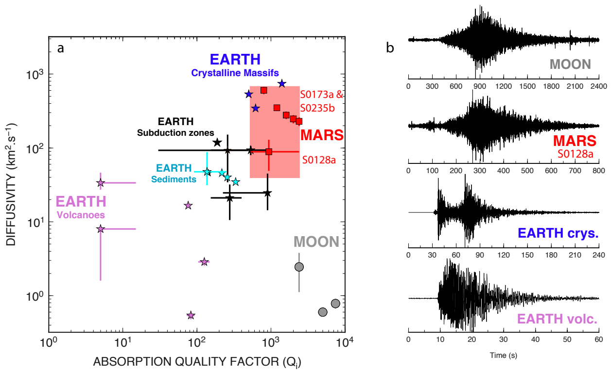
Figure S3-12: Comparison of seismic scattering and attenuation on Earth, Moon, and Mars. a: Diffusivity and attenuation. Except for Mars and the Moon, the diffusivity is given in the 1-2 Hz frequency band. See the text for details. b: Several illustrative seismograms showing the impact of the geological environment on the anatomy of the seismogram. Figure compiled after the following articles: Mayeda et al. (1992), Ugalde et al. (2010), Wegler (2003), Del Pezzo et al. (2001), Badi et al. (2009), Hoshiya et al. (2001), Yoshimoto et al. (2006), Lenzikov (2007), Chung et al. (2009), Lacombe et al. (2003), Sens-Schönfelder et al. (2009), Sens-Schönfelder & Wegler (2006), Carcolé & Sato (2010), Pujades et al. (1997), Dainty et al. (1974), Gillet et al. (2017), Menina (2019).
