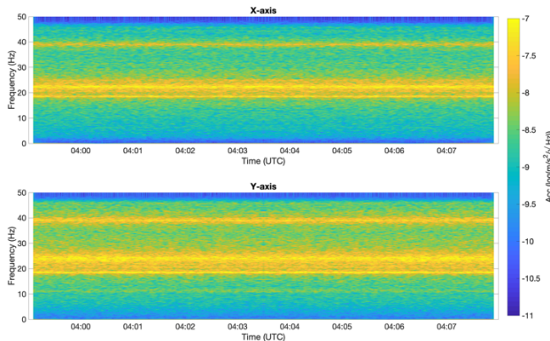
Figure S2-1a: Spectrogram of Martian SEIS data from January, 4 on X and Y axes, by using the 3 SPs and 3 VBBs signals. The 39 +/- 1 Hz resonance is due to the LVL structure.
