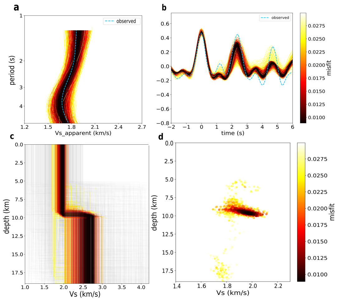
Figure S4-9. Results of the inversion of apparent S-wave velocities and the first 6 s of the radial RF of S0173a (MPS deglitching) for a layer-over-a-half-space model. a Fit to apparent S-wave velocity curve b Fit to RF waveform c Resulting velocity models. Gray lines indicate models also investigated which have a larger misfit than the colored range. d Trade-off plot between depth and S-wave velocity of the first layer. Minimum, maximum and best fit S and P velocities for the two layers are provided in Supplementary Table 3 .
